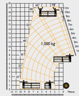
540-180 HiViz Man platform Stabilisers extended
